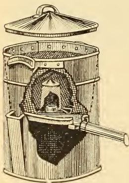
FIG. 36.—Excelsior wax extractor.
