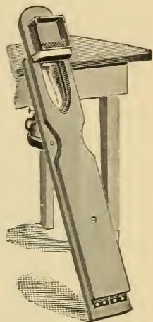
FIG. 40.—The Daisy foundation fastener. (From Gleanings.)
