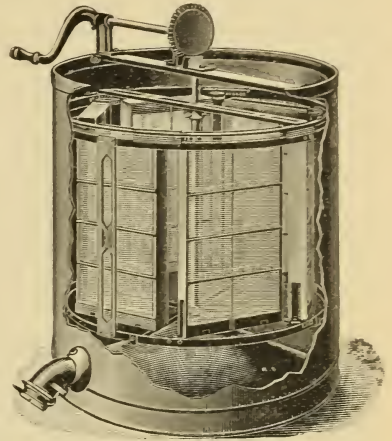
FIG. 33.—Williams' automatic reversible honey extractor.
